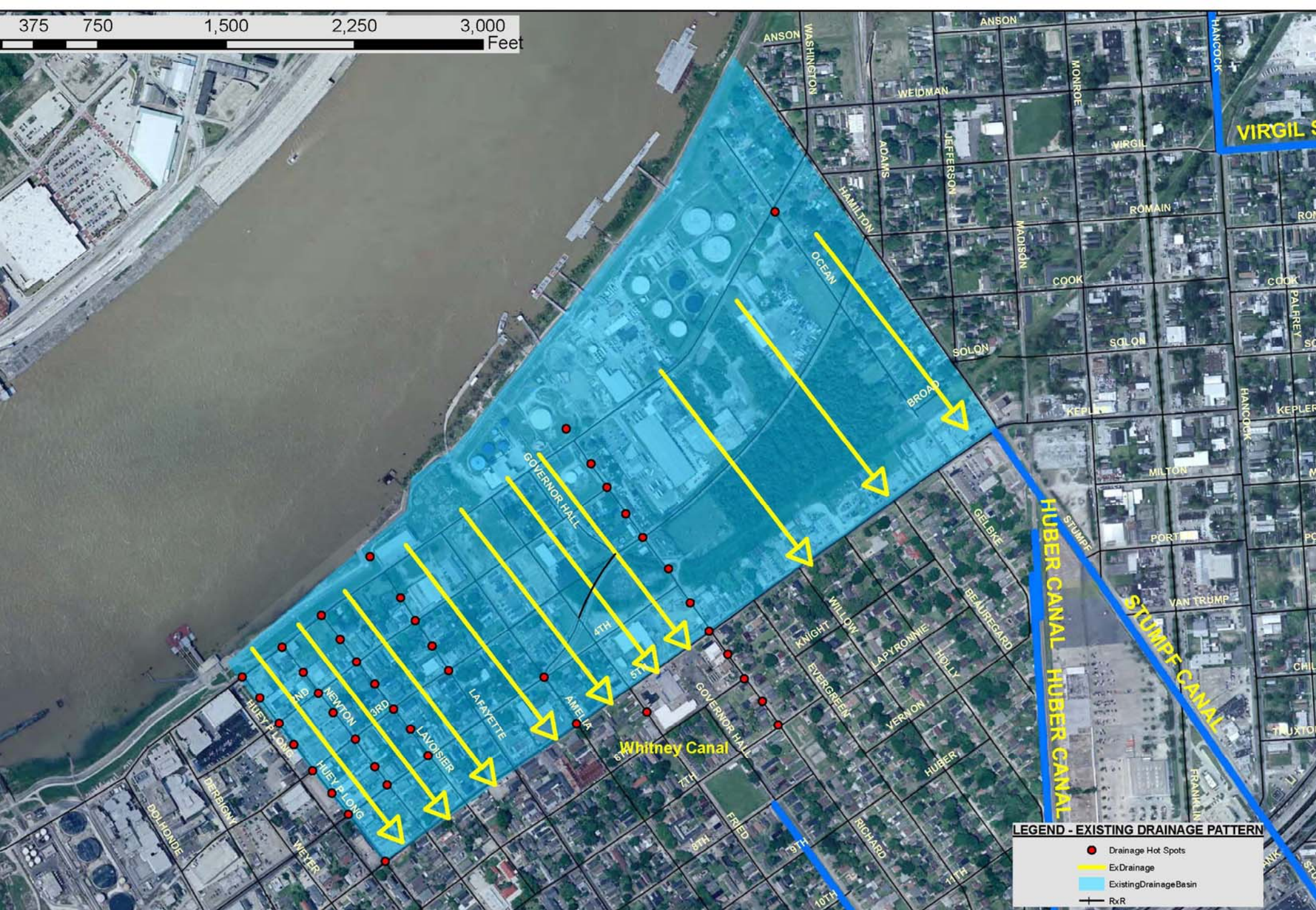
Huey P. Long Ave. to Hamilton St. Drainage Study Existing Drainage Pattern
