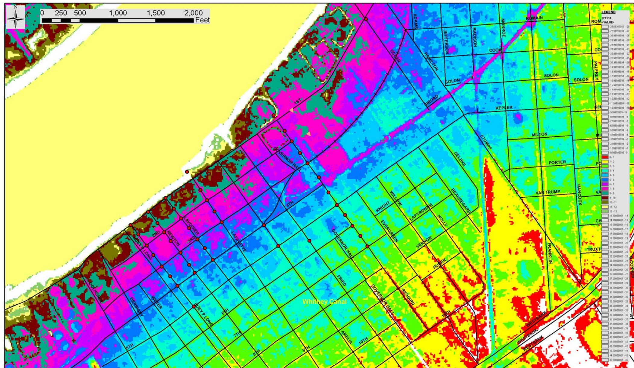
Huey P. Long Ave. to Hamilton St. Drainage Study Proposed Capital Improvement & D.P.W. Projects Lidar (Light Detection And Ranging)
